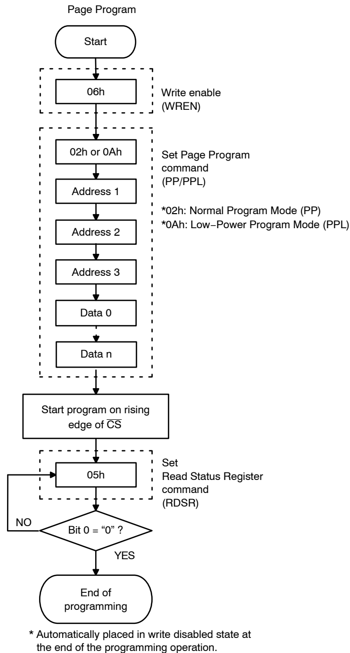
Figure 41. Page Program Flowcharts
