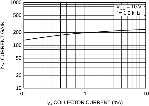
Figure 15. Current Gain
