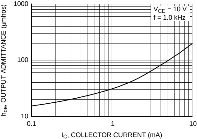
Figure 14. Output Admittance
