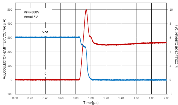
Figure 10. Turn-on Waveform T_J = 100^\circ\text{C} , V_{CC} = 300\text{ V}
