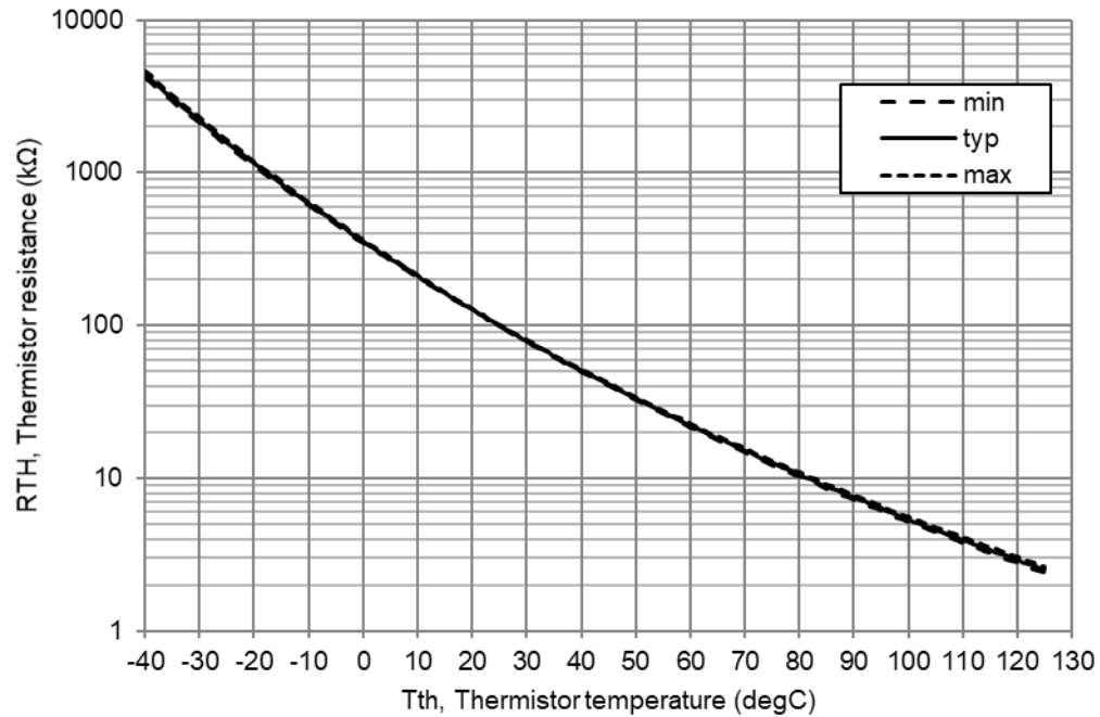
Figure 13. Thermistor Resistance versus Thermistor Temperature
