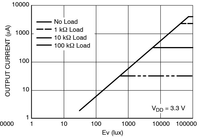
Figure 6. Output Current vs. Ev (Medium Gain)
