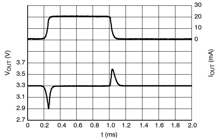
Figure 31. Load Transients, 3.3 V Version, I_{\text{OUT}} = 1 - 20 \text{ mA} , t_{\text{R}} = t_{\text{F}} = 50 \mu\text{s} , V_{\text{IN}} = 6.3 \text{ V}
