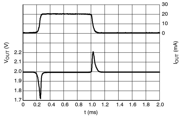
Figure 30. Load Transients, 2.0 V Version, I_{\text{OUT}} = 1 - 20 \text{ mA} , t_{\text{R}} = t_{\text{F}} = 50 \mu\text{s} , V_{\text{IN}} = 5.0 \text{ V}
