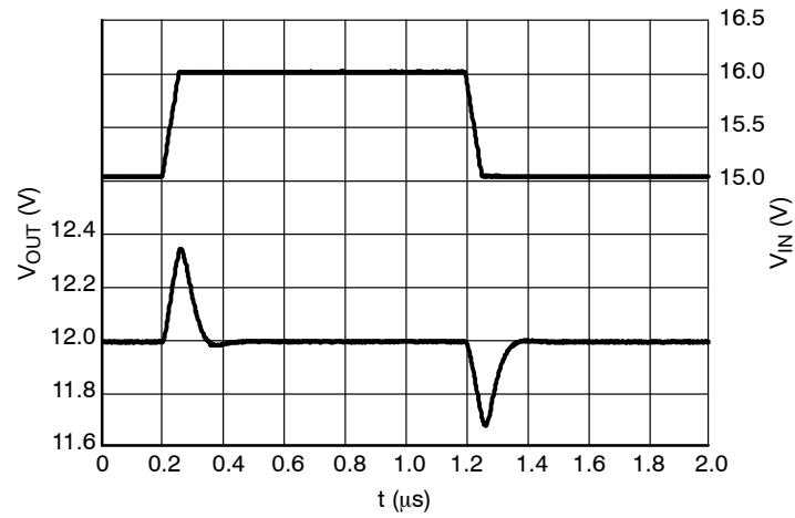
Figure 29. Line Transients, 12.0 V Version, t_{\text{R}} = t_{\text{F}} = 50 \mu\text{s} , I_{\text{OUT}} = 1 \text{ mA}
