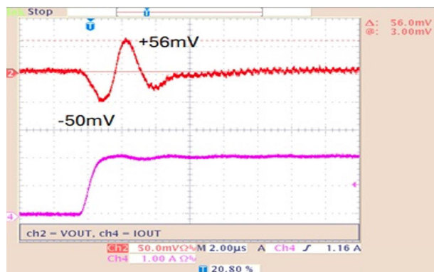
Figure 24. TRANSIENT_ENHANCEMENT bit enabled, 10 mA \leftrightarrow 2 A, Slew Rate = 2 A/ \mu s
