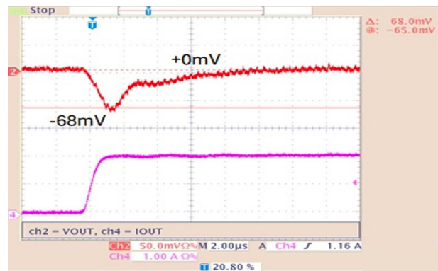
Figure 25. TRANSIENT_ENHANCEMENT bit disabled, 10 mA \leftrightarrow 2 A, Slew Rate = 2 A/ \mu s
