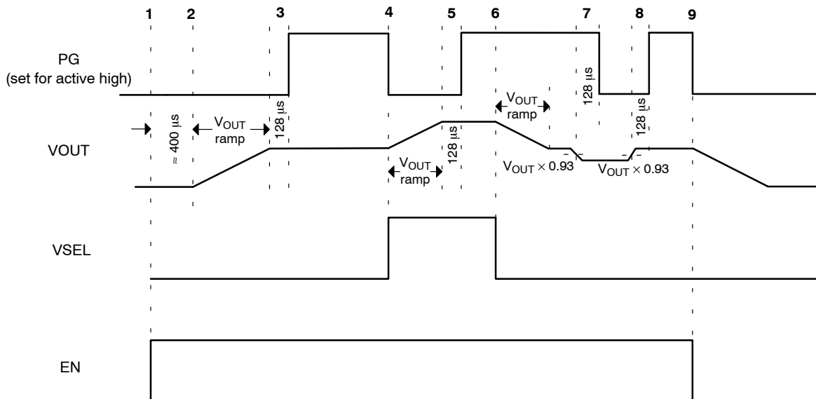
Figure 27. PG Operation
