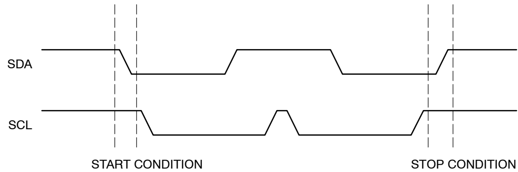
Figure 13. Start/Stop Condition
