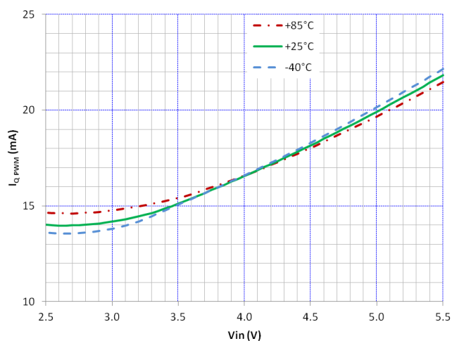
Figure 21. I_Q\text{ PWM} vs V_{IN} and Temperature
