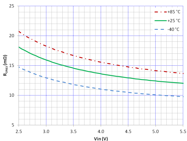
Figure 17. LSS R_{ON} vs V_{IN} and Temperature
