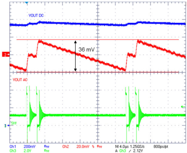
Figure 25. PFM Ripple
