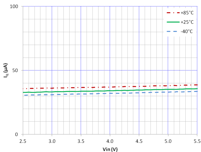
Figure 20. I_Q\text{ PFM} vs V_{IN} and Temperature
