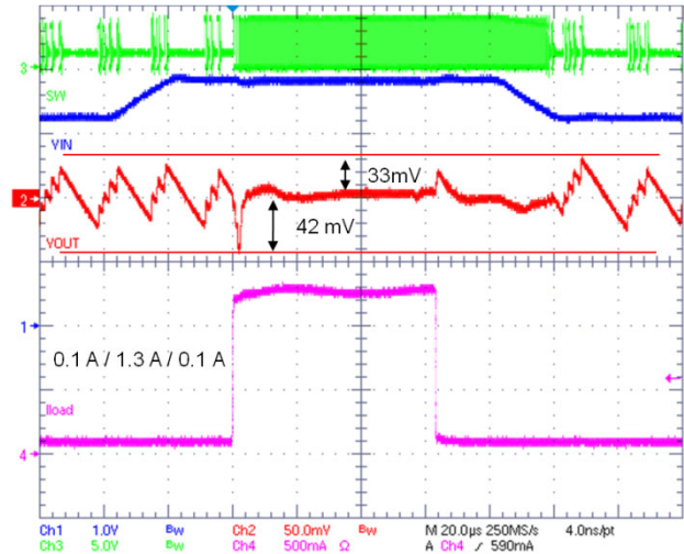
Figure 28. Transient Load 0.2 to 1.5 A – Single Shot Transient Line 3.3 to 3.9 V – Auto Mode
