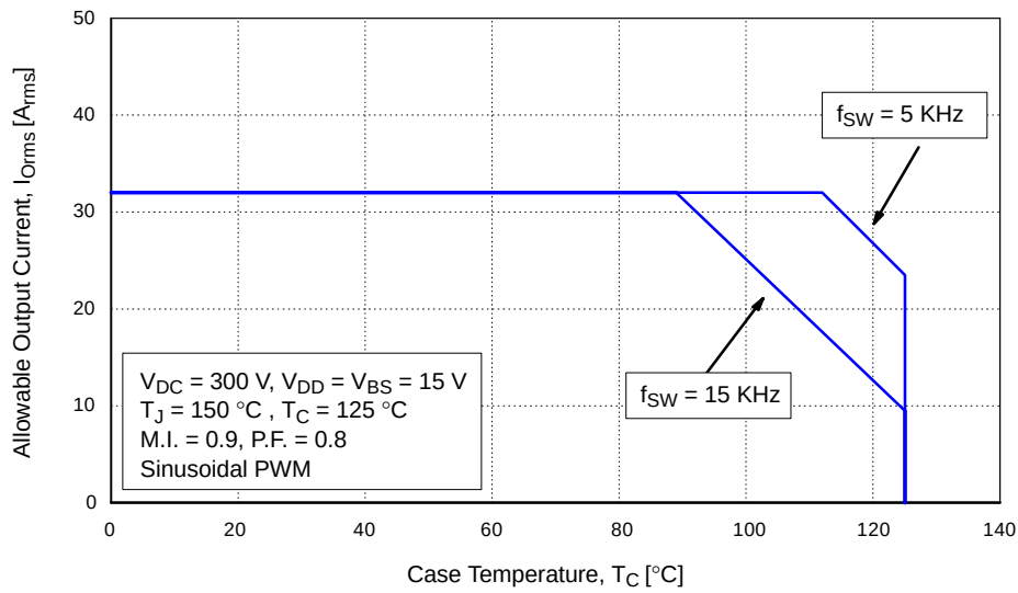
Figure 7. Allowable Maximum Output Current
