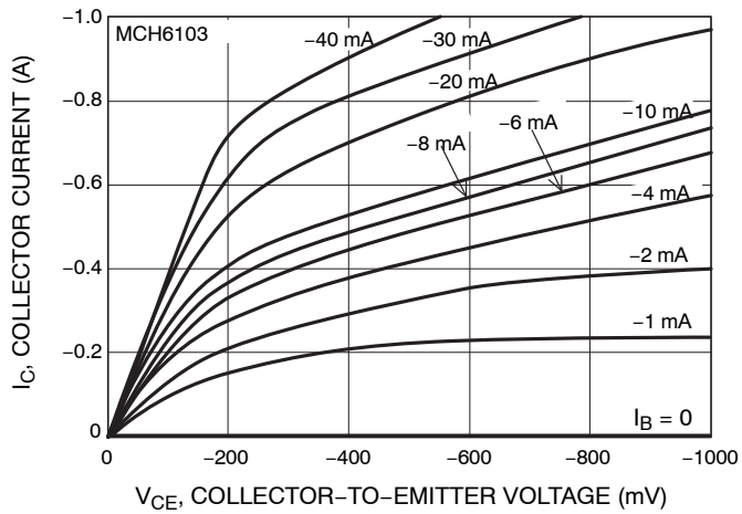
Figure 2. I_C - V_{CE}
