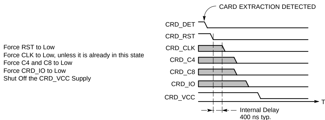
Figure 8. Card Power Down Sequence
