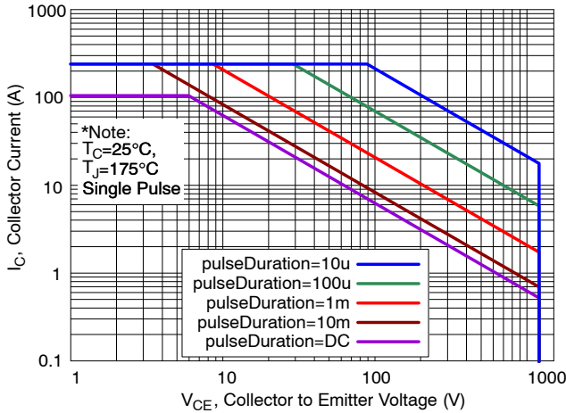
Figure 9. SOA Characteristics
