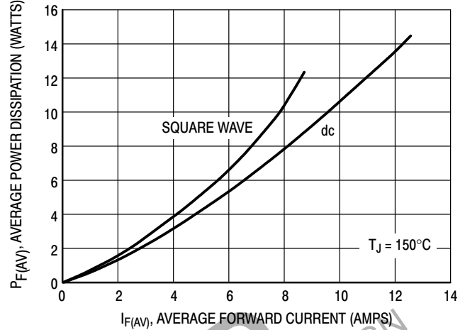
Figure 5. Power Dissipation
