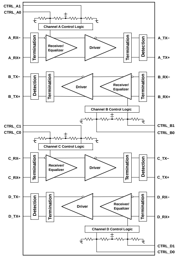
Figure 1. Logic Diagram
