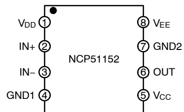
NCP51152xB
