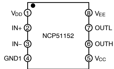
NCP51152xA
