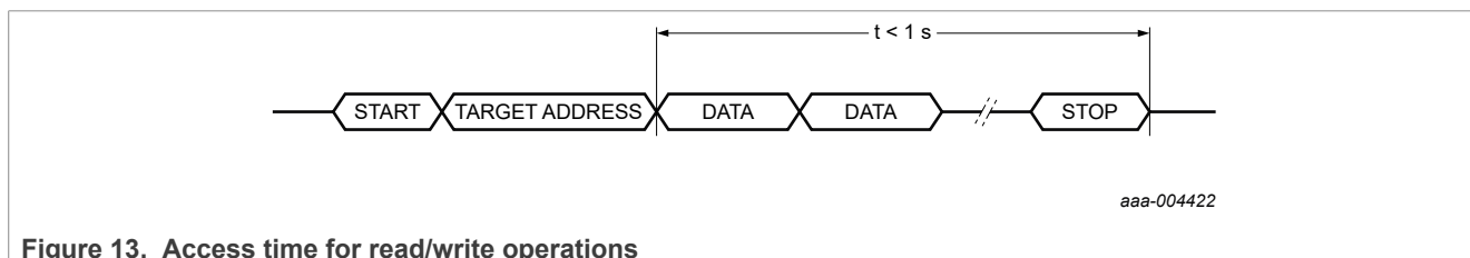
Figure 13. Access time for read/write operations
