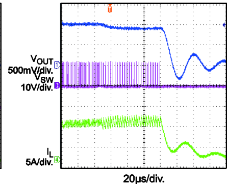
OCP Protection NB650, Latch-Off Version
