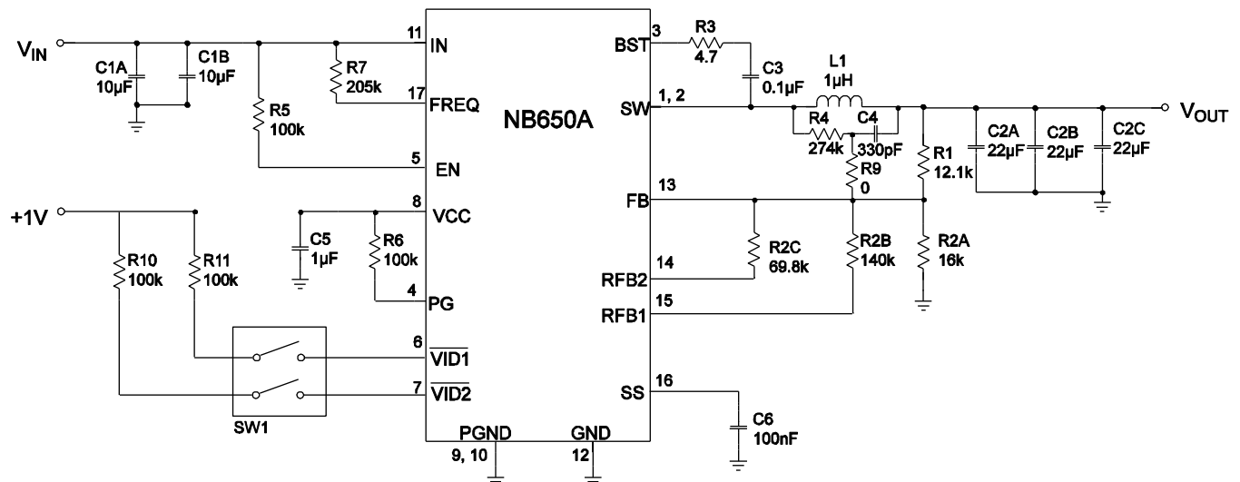
Figure 13: Typical Application with Low-ESR Ceramic Capacitor
