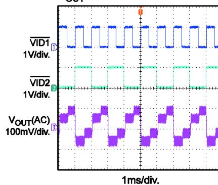
VID On-the-fly I_{OUT} = 0.3A F_{VID1} = 1kHz , F_{VID2} = 0.5kHz , V_{OUT} = 1.05V/1.1V/1.15V/1.2V
