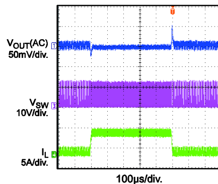
Transient I_{OUT} = 0.6A-5.4A@2.5A/\mu s , F_{SW} = 530kHz , C_{OUT} = 3 \times 22\mu F
