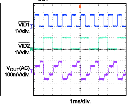
VID On-the-fly I_{OUT} = 6A F_{VID1} = 1kHz , F_{VID2} = 0.5kHz , V_{OUT} = 1.05V/1.1V/1.15V/1.2V
