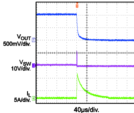
Short Circuit Protection NB650, Latch-Off Version
