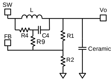
Figure 10: Simplified Ceramic Capacitor Circuit
