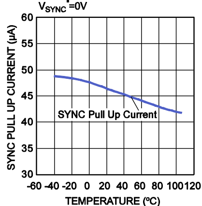
SYNC Pull Up Current vs. Temperature
