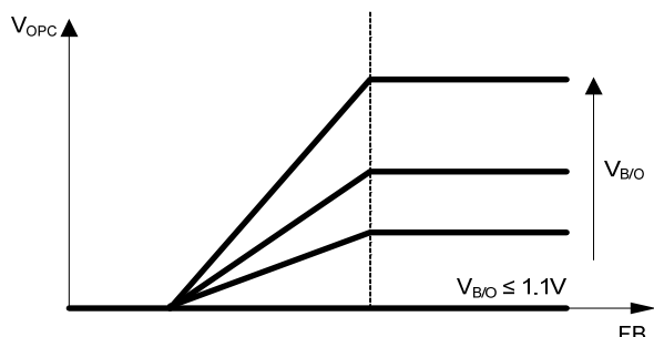
Figure 9: Compensation Voltage vs. FB and B/O
