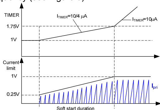
Figure 6: Soft Start
