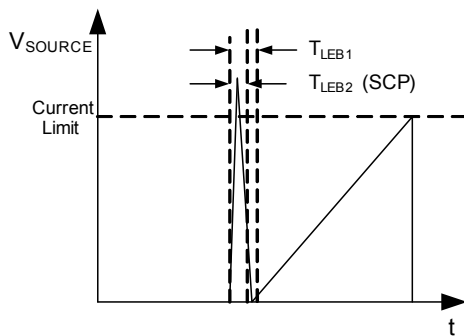
Figure 10: Leading-Edge Blanking
