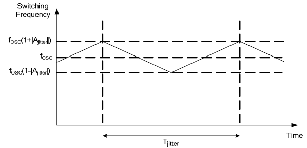
Figure 3: Frequency Jittering
