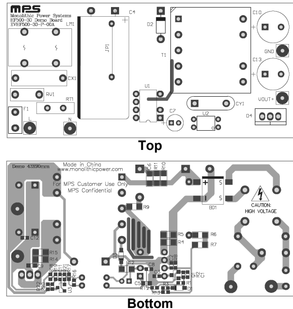
Figure 13: Recommended PCB Layout
