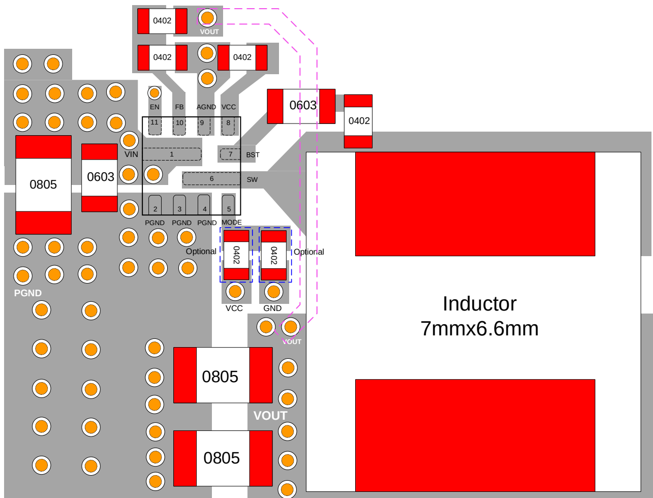
Figure 10: Recommended PCB Layout
