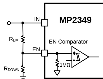
Figure 7: Adjustable UVLO
