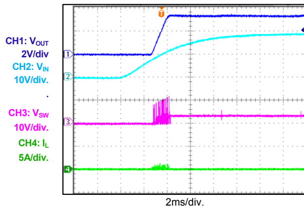
Startup through Input Voltage
