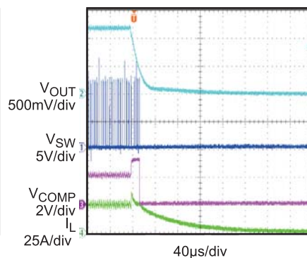
Over-current Protection
