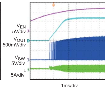
Start up through IN
