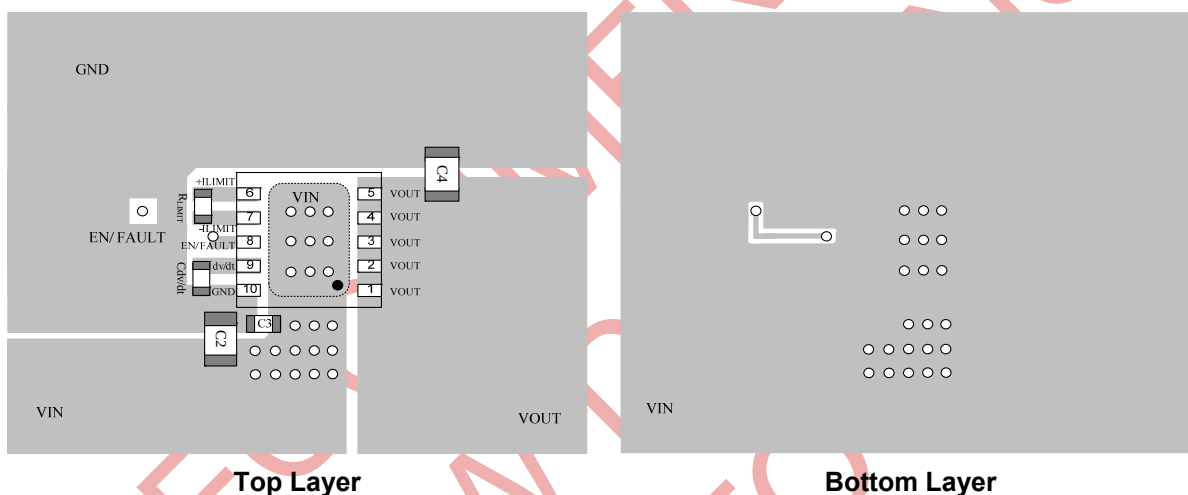
Figure 4—PCB Layout
