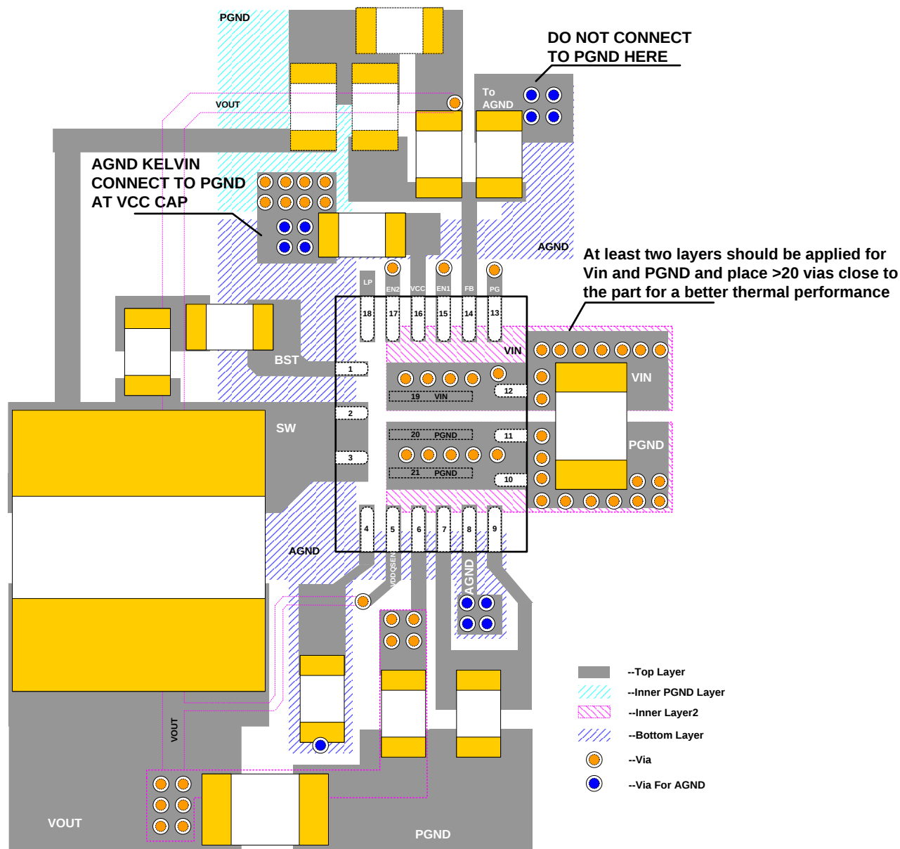
Figure 13—Recommend Layout
