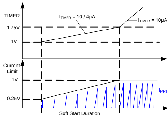
Figure 6: Soft Start
