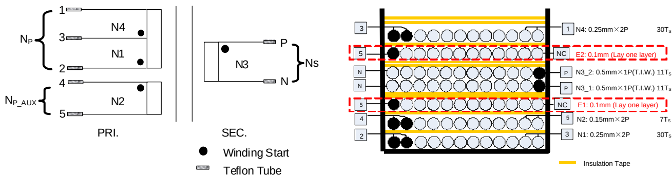
Connection Diagram
