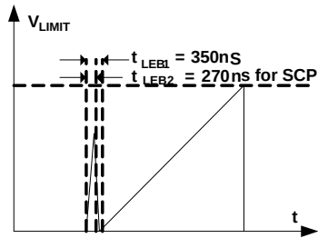
Figure 10: Leading-Edge Blanking
