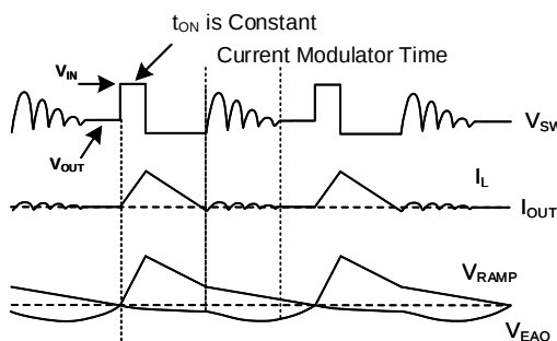
Figure 4: Light-Load Operation
