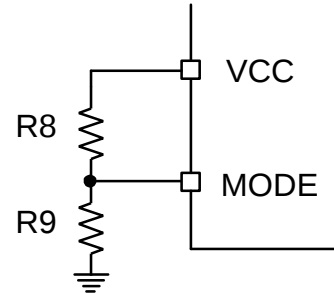
Figure 5: MODE Configuration
