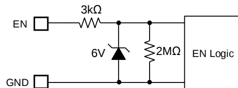
Figure 6: Zener Diode between EN and GND
