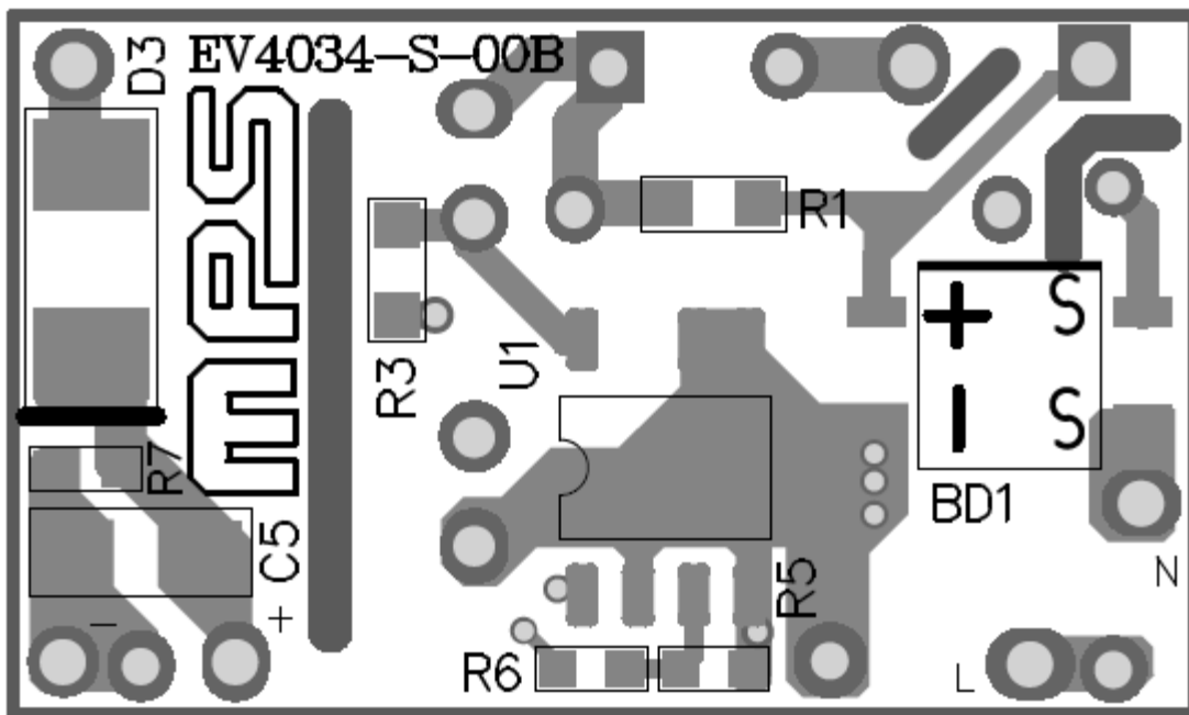
Figure 3: Bottom Layer
