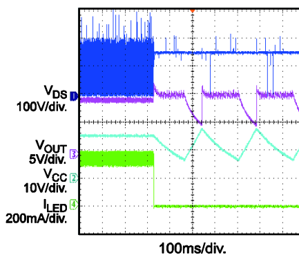
Lamp Open Protection
