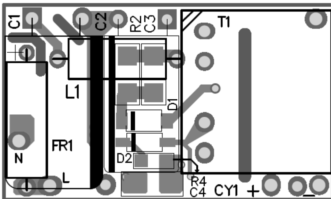
Figure 2: Top Layer
