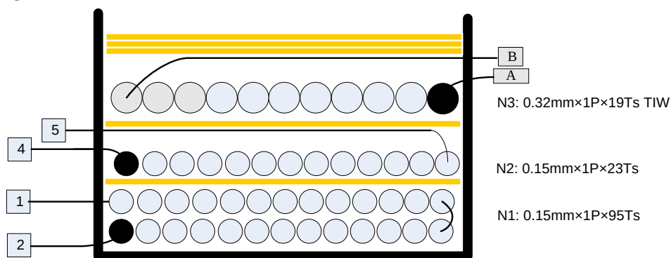
Figure 5: Winding Diagram
