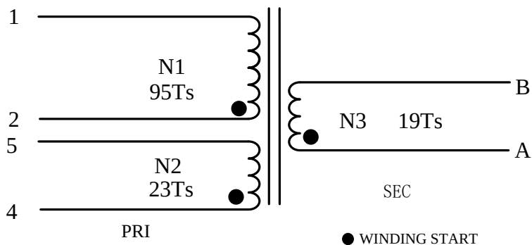
Figure 4: Transformer Diagram
