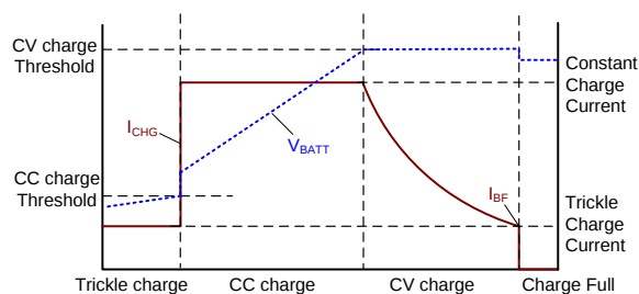
Figure 2: Li-Ion Battery Charge Profile
