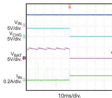
Short Charger Circuit Protection
