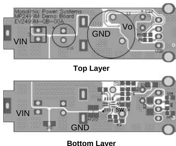
Figure 9: Recommended PCB Layout
