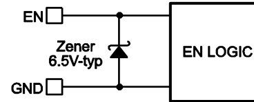
Figure 2: 6.5V Type Zener Diode
