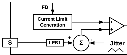
Figure 9: Frequency Jittering
