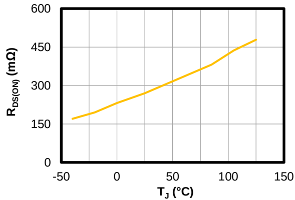
Drain-to-Source On Resistance vs. Junction Temperature
