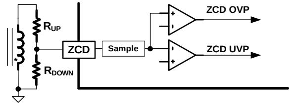
Figure 10: ZCD OVP and ZCD UVP Circuit
