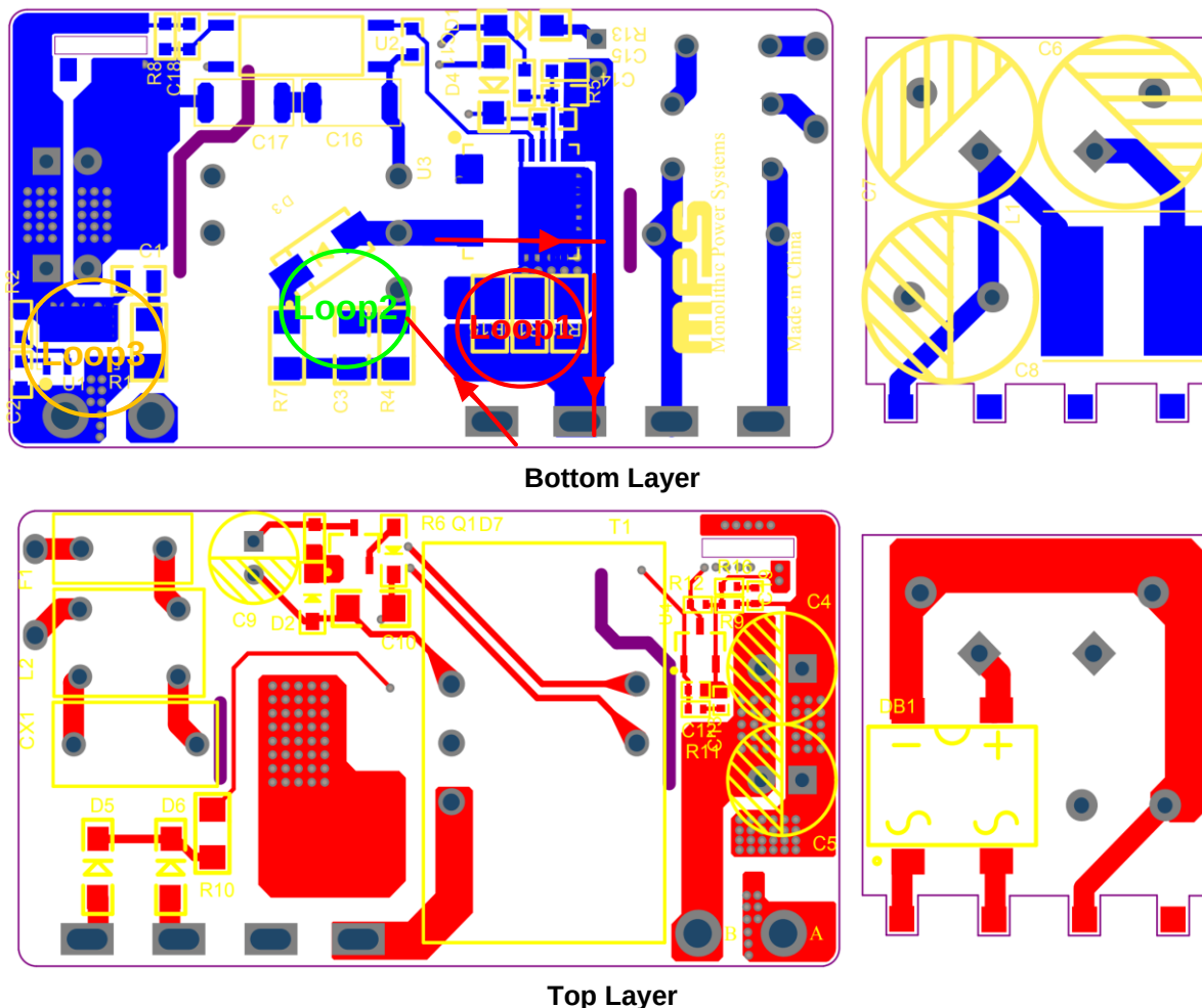
Figure 16: Recommended PCB Layout
