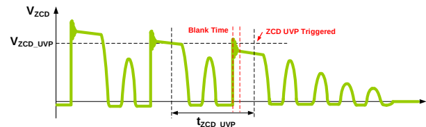
Figure 12: ZCD UVP Voltage Sampling
