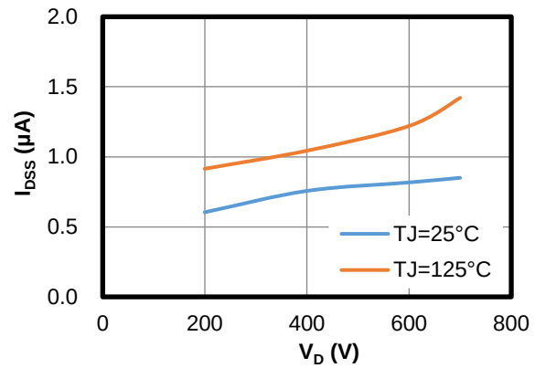
Drain-to-Source Leakage Current vs. Drain Voltage
