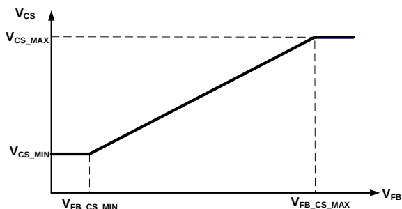
Figure 5: Current Limit Modulation vs. V_{FB}
