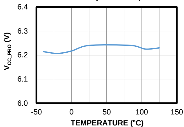
V_{CC} Release Level after Auto-Recovery vs. Temperature
