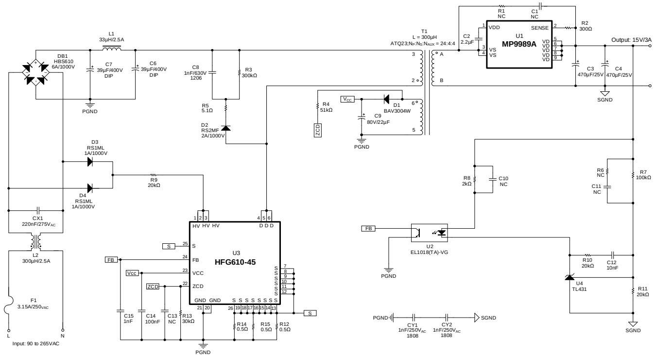
Figure 17: Typical Application Circuit (45W Output and Universal Input)
