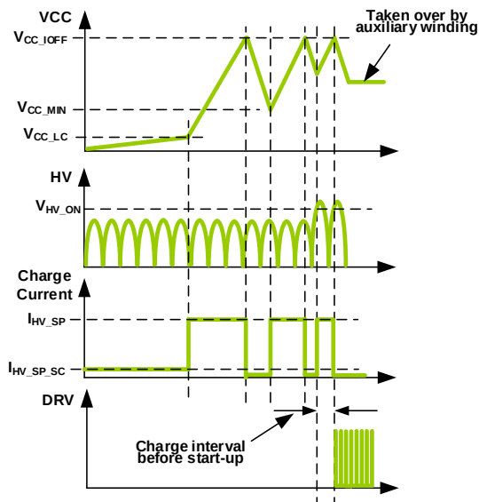
Figure 2: Start-Up with Brown-In and Brownout Detection
