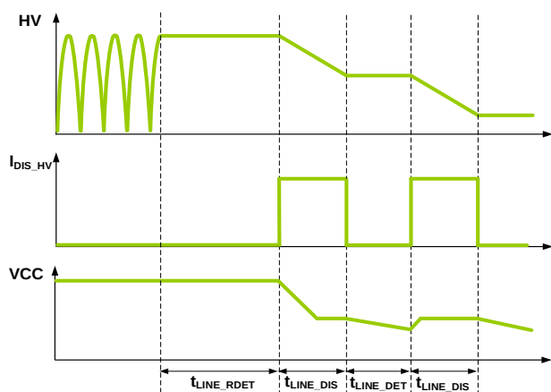
Figure 8: X-Capacitor Discharger
