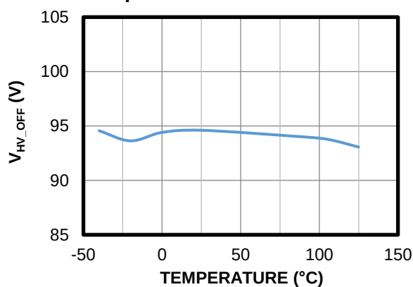
Brownout Threshold vs. Temperature
