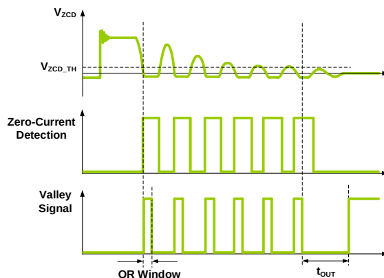
Figure 6: QR Signal Generation
