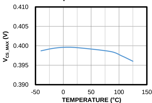
Current-Sense Maximum Voltage vs. Temperature
