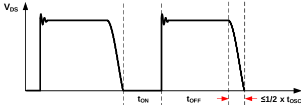
Figure 15: Switching Period in Low Line
