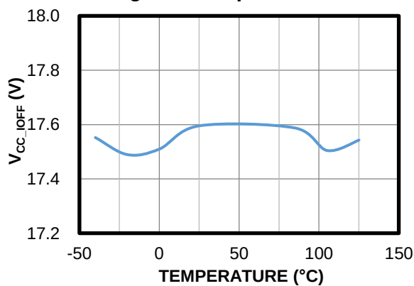
HV Supply Current Turn-Off Voltage vs. Temperature
