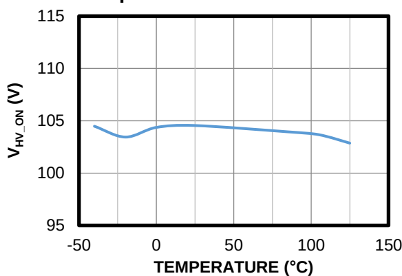
Brown-In Threshold vs. Temperature
