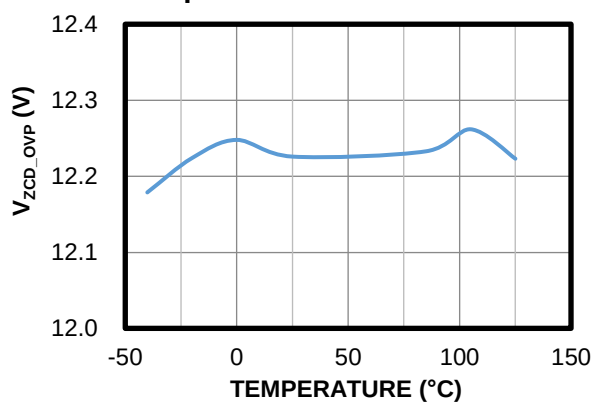
ZCD OVP Threshold vs. Temperature
