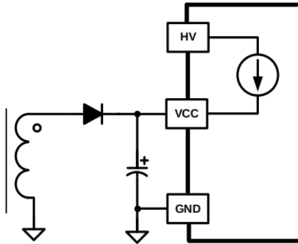
Figure 13: Start-Up Circuit
