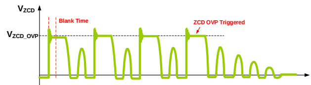
Figure 11: ZCD OVP Voltage Sampling
