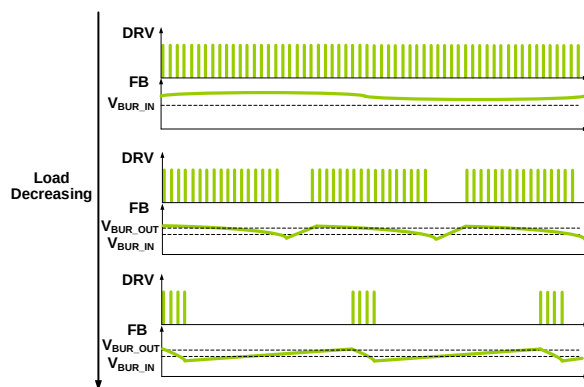
Figure 7: Forced Burst Mode
