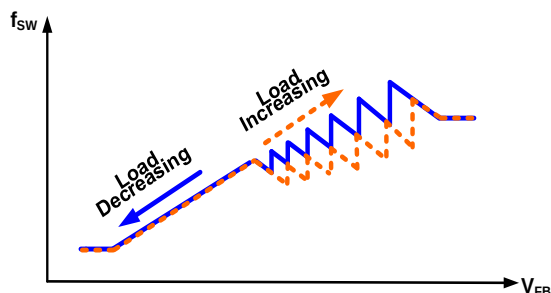
Figure 4: f_{SW} vs. V_{FB}
