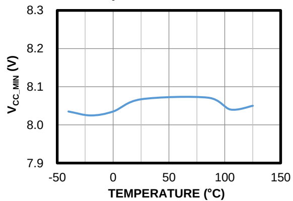
VCC Minimum Operating Voltage vs. Temperature
