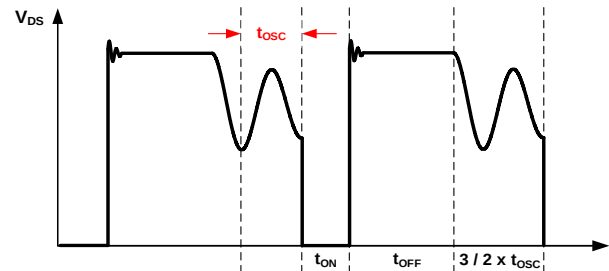
Figure 14: Switching Period in High Line
