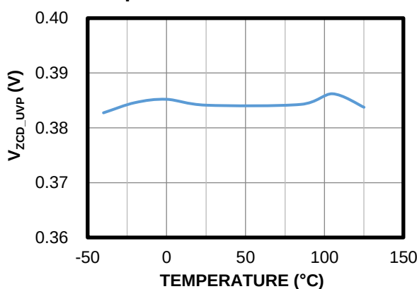
ZCD UVP Threshold vs. Temperature
