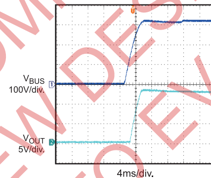
Turn-On Delay
