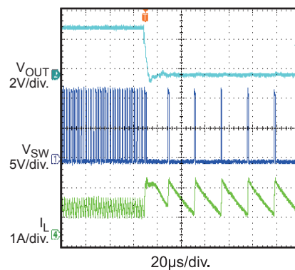
Short Circuit Protection I_{OUT} = 1A
