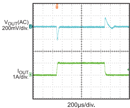
Load Transient Response I_{OUT} = 0A \text{ to } 1A, 1.6A/\mu s
