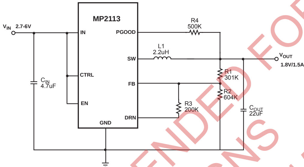
Figure 3-Typical Application Circuit
