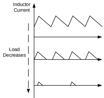
Figure 2: AAM Mode and PWM Mode
