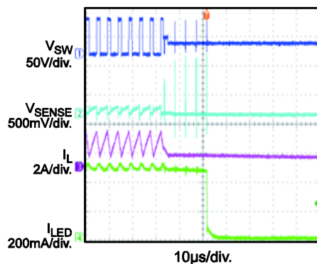
Short-Inductor Protection
