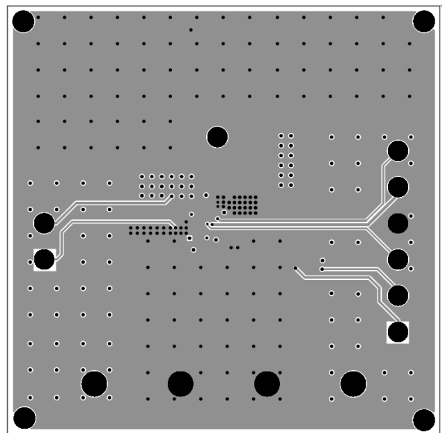
Figure 4: Inner Layer2
