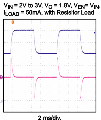
Line Transient
