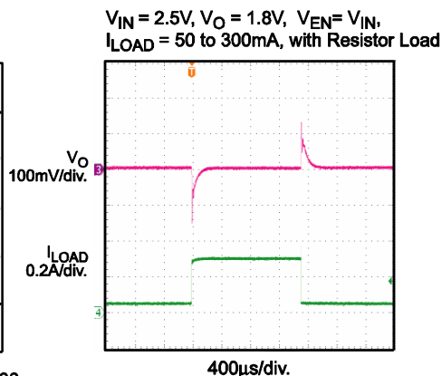
Load Transient
