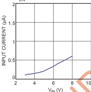
Shutdown Current vs. Input Voltage V_{EN}=Low
