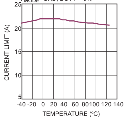
Current Limit vs. Temperature V_{MODE}=GND , DUTY=40%
