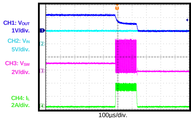
Short-Circuit Entry
