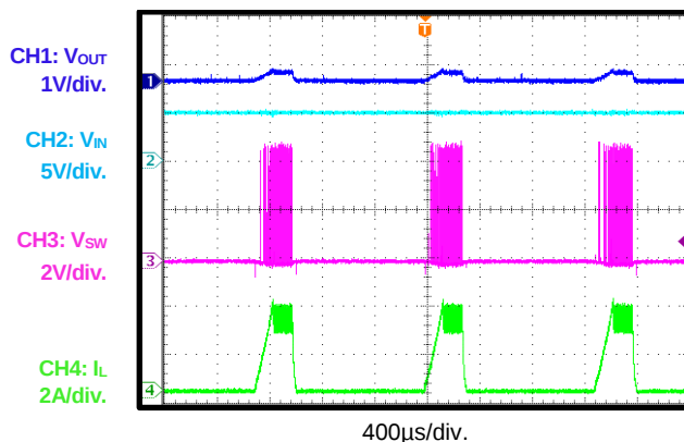
Short-Circuit Protection
