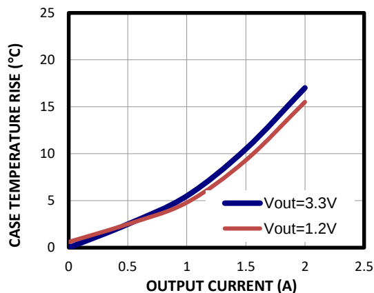
Case Temperature Rising
