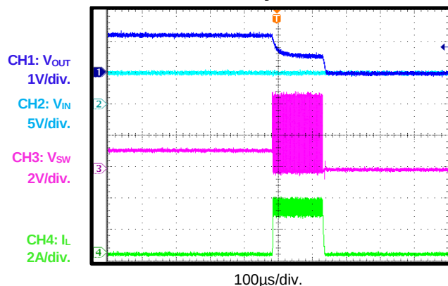
Short-Circuit Entry
