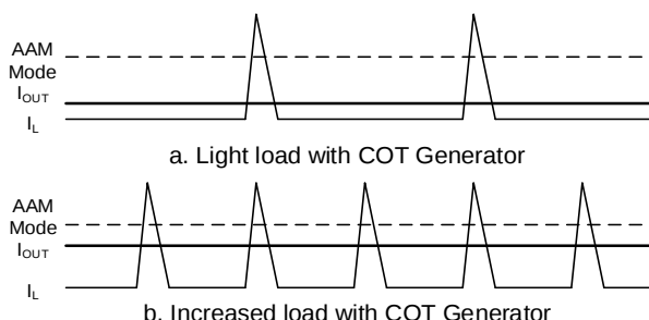
Figure 7: On-Time Control t_{ON}
