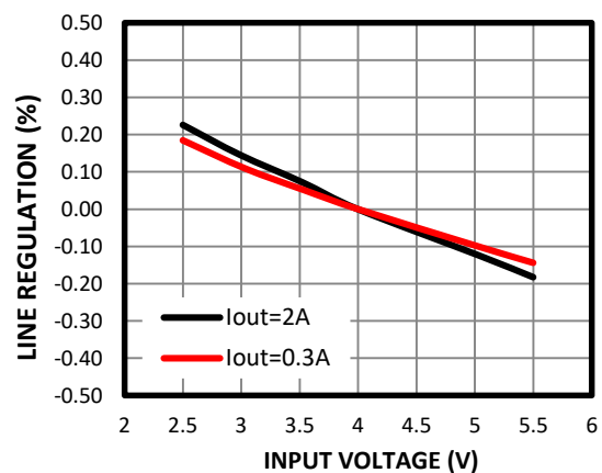
Line Regulation
