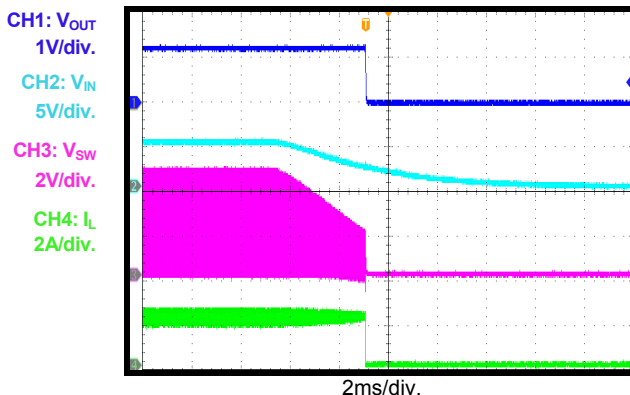
V_{IN} Shutdown
