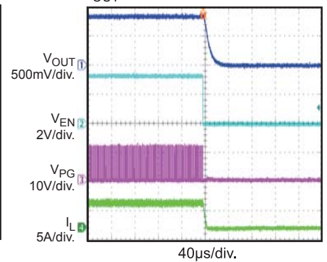
Power Good through EN Shutdown
