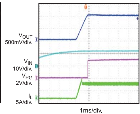
Power Good through VIN Startup
