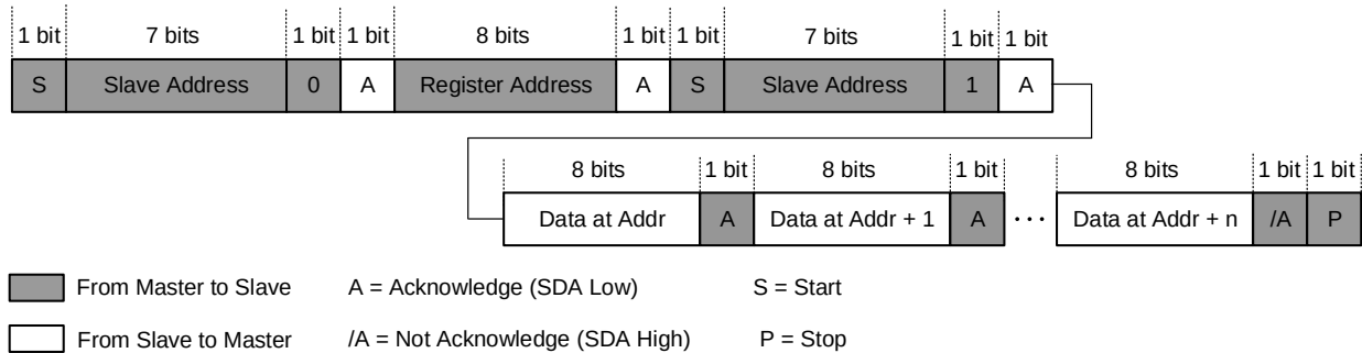
Figure 18: Multi-Read
