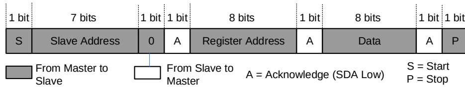
Figure 15: Single Write
