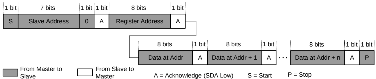
Figure 17: Multi-Write
