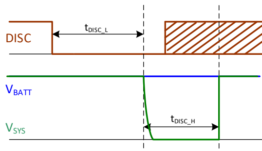
Figure 9: System Auto-Reset
