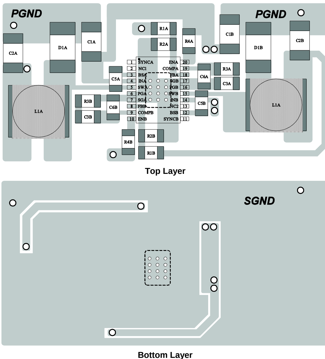
Figure3—PCB Layout
