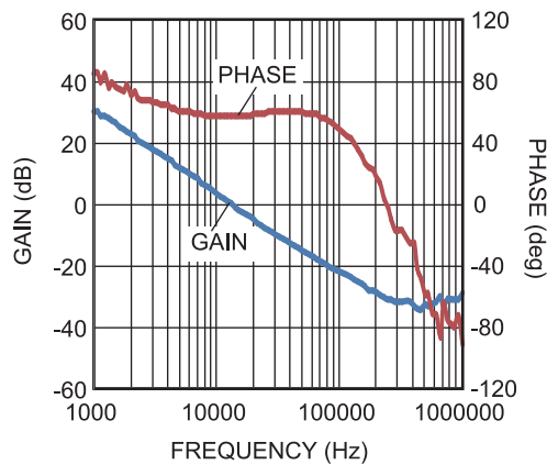
Bode Plot
