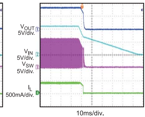
V_{IN} Shutdown
