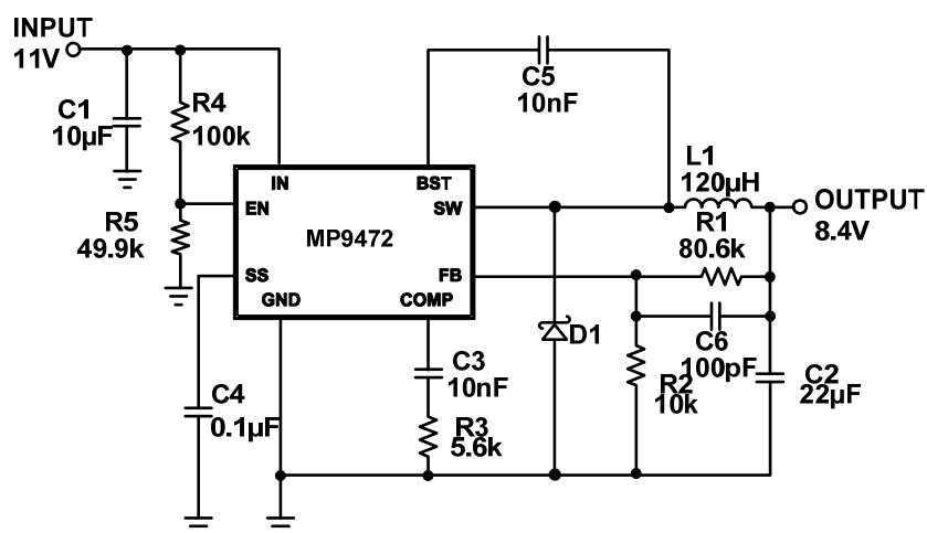
Figure 3: MP9472 with 8.4V Output, 22μF Ceramic Output Capacitor
