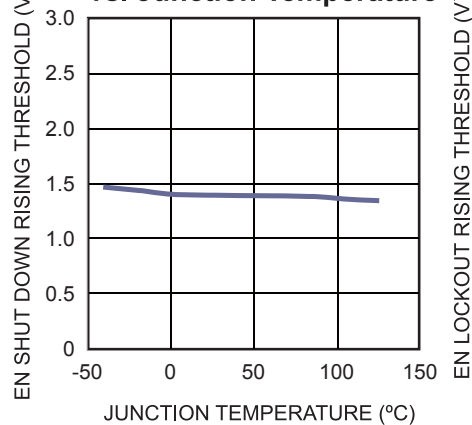
EN Shutdown Rising Threshold vs. Junction Temperature
