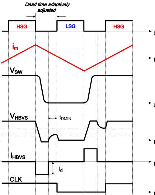
Figure 29: Operation Waveform of ADTA
