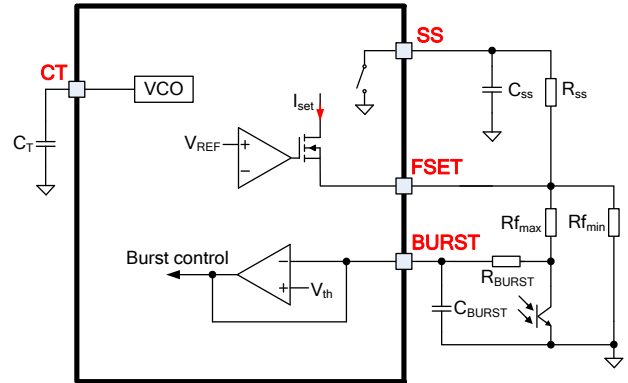
Figure 36: Burst-Mode Operation Set-Up
