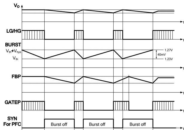
Figure 37: Burst-Mode Operation
