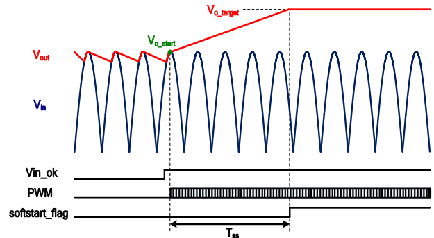
Figure 24: Soft-Start Sequence
