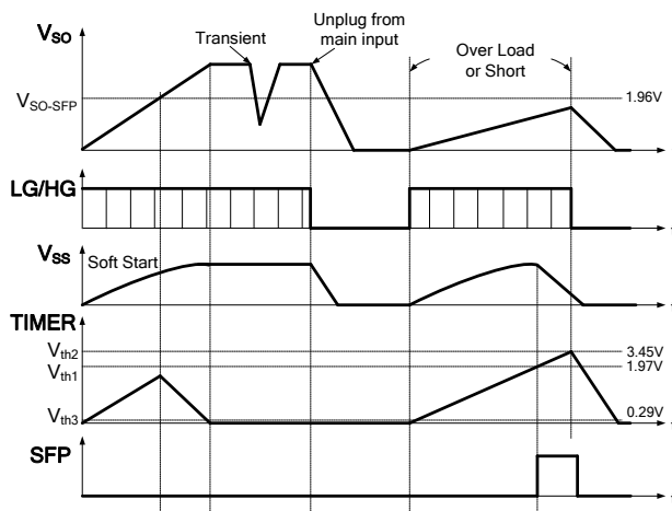
Figure 38: SFP Timing
