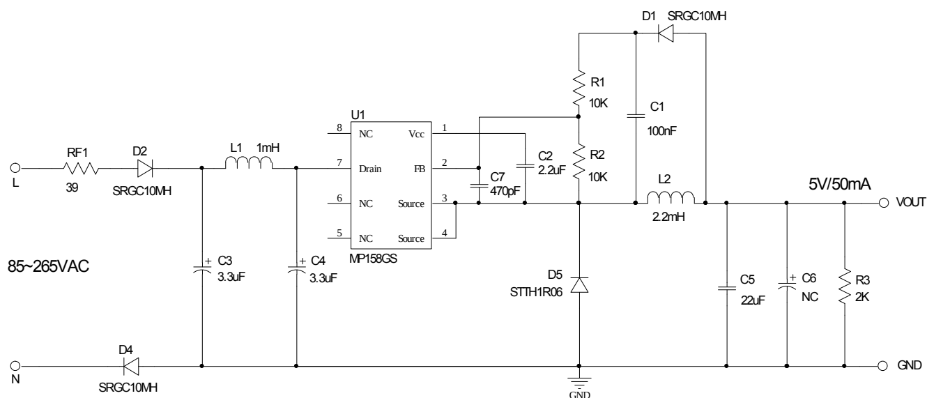
Figure 1—Schematic
