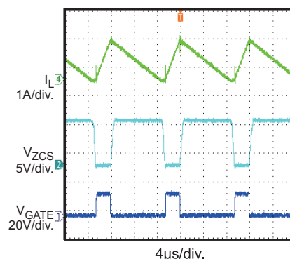
Zero-Current Sensing
