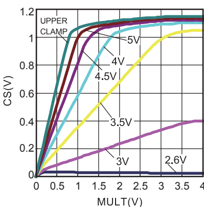
Multiplier Characteristic
