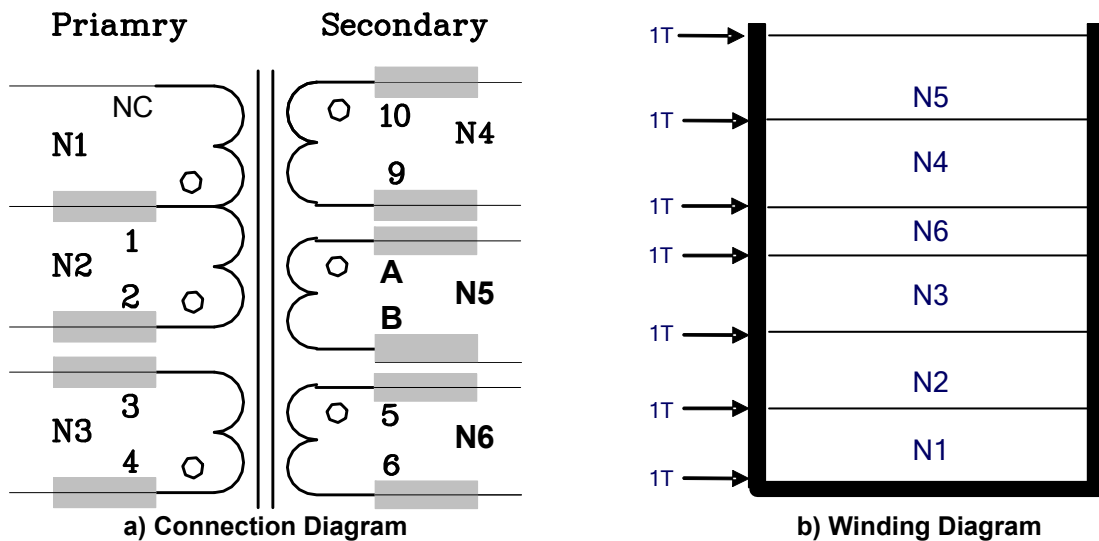
Figure 12: Transformer Structure
